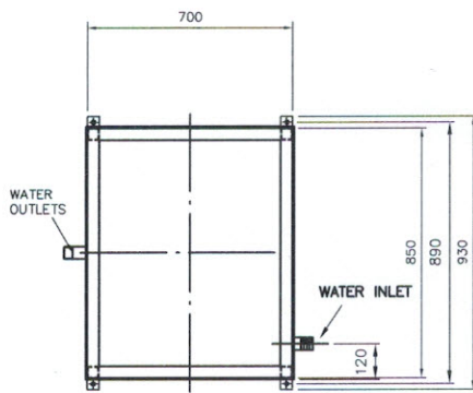
PLAN VIEW ROOF PANELLING WITH INSULATION OMITTED TO SHOW INTERNAL DETAIL
