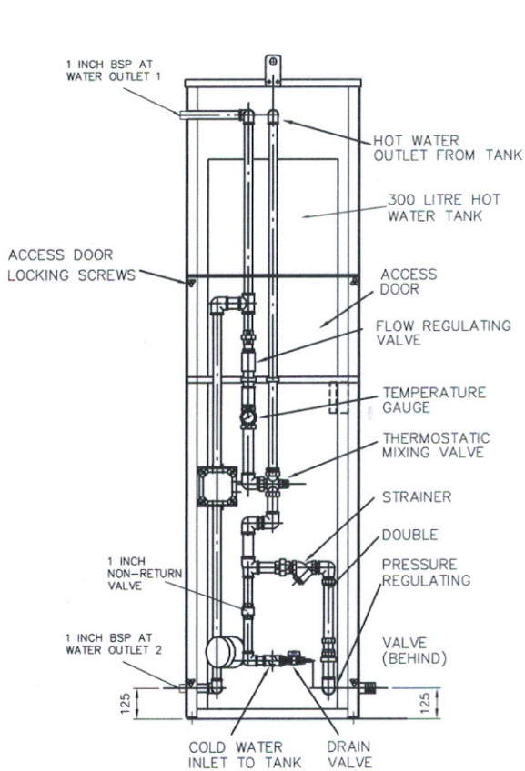
SIDE VIEW SIDE/DOOR PANELLING WITH INSULATION OMITTED TO SHOW INTERNALS
